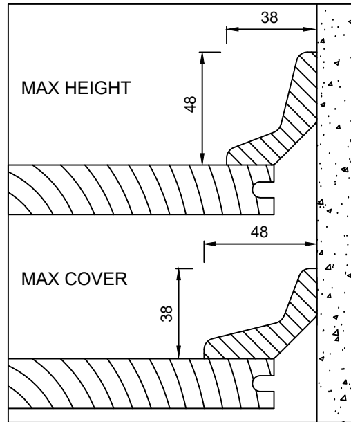
JUNCKERS COMBI SKIRTING
